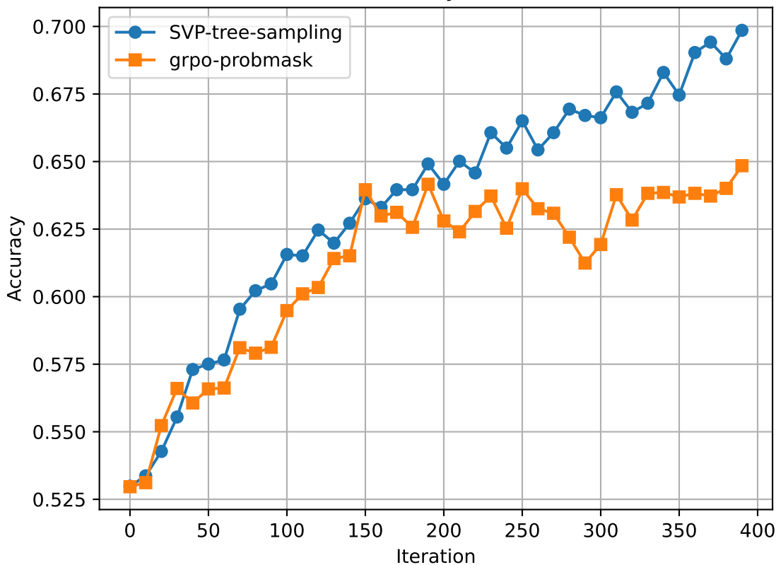
Validation Accuracy Over Iterations
